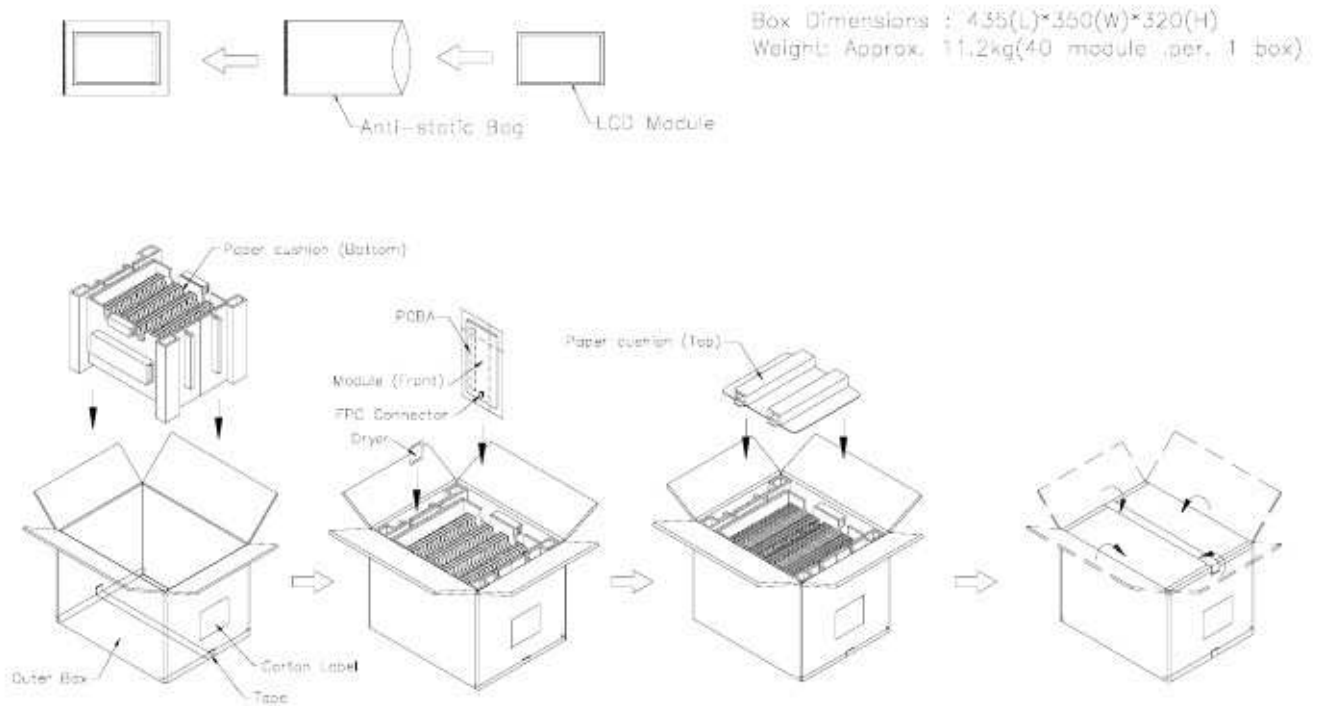
Figure. 10-1 Packing method
