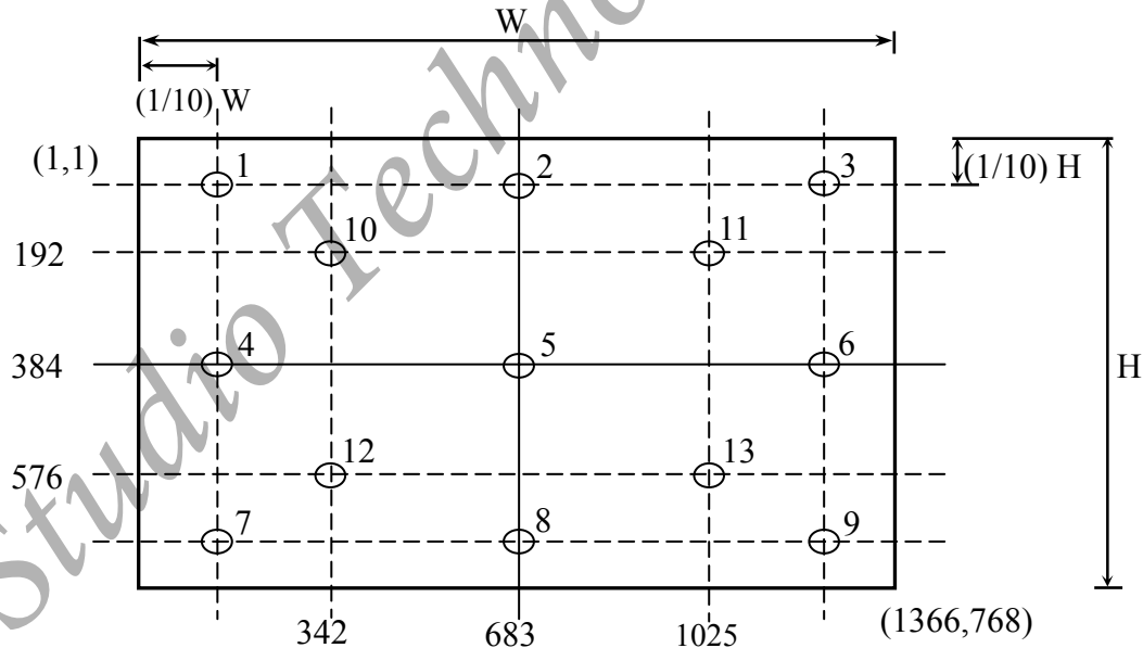
Fig.1 Measure point
