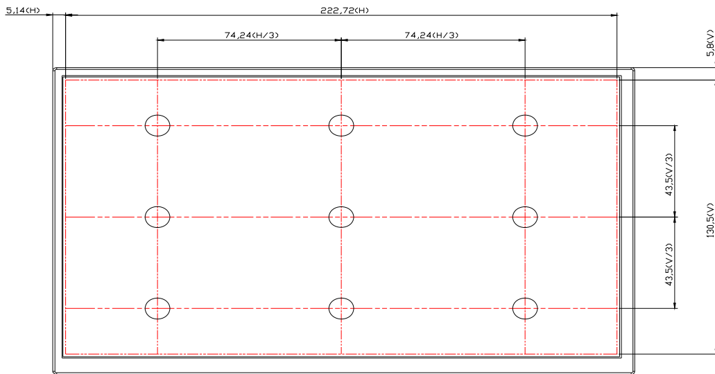
Fig8-1 Measuring point
